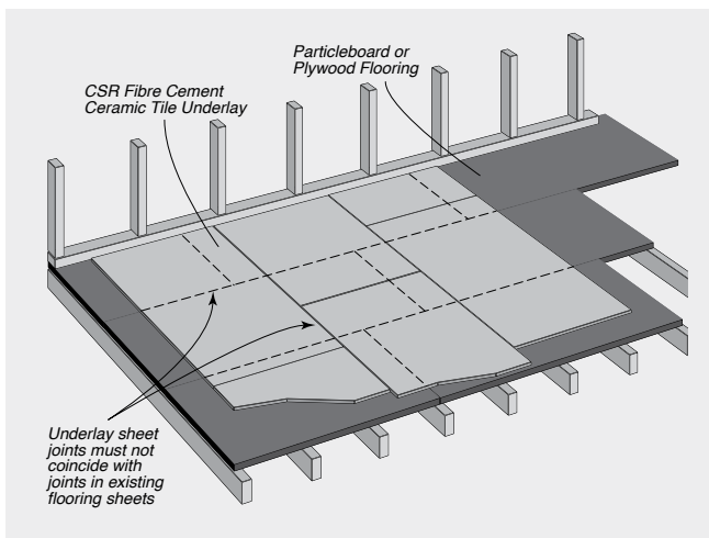
FIGURE 4.01 System Overview
