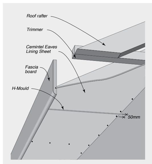
FIGURE 2.05 Eaves Lining
