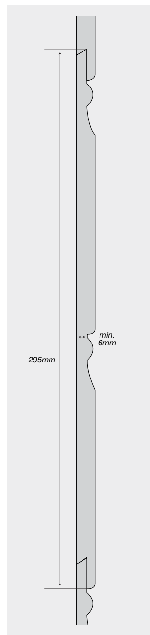
FIGURE 3.17 Profile
