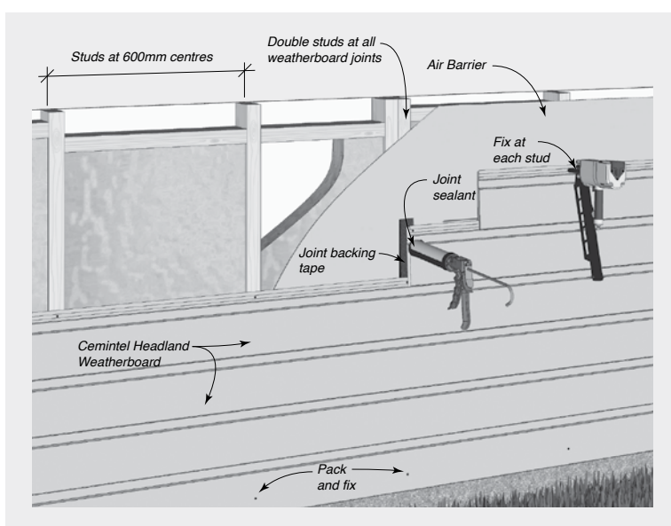
FIGURE 3.18 System Overview
