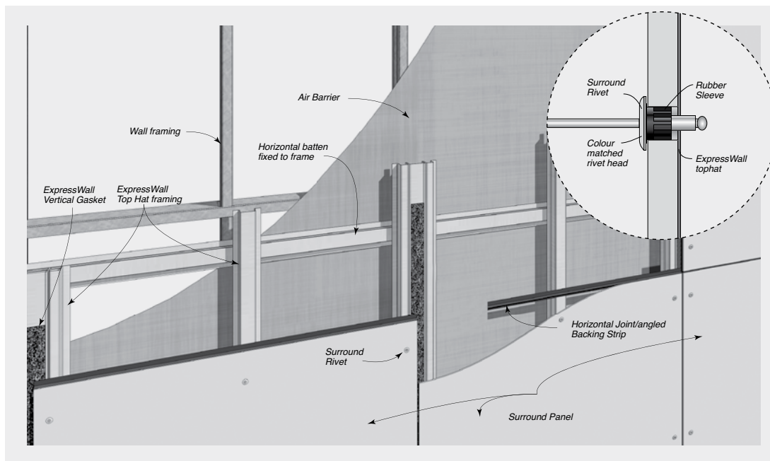
FIGURE 3.02 System Overview
