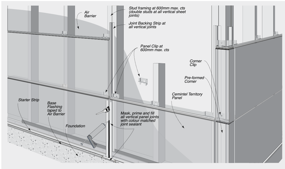
FIGURE 3.04 Horizontal Installation
