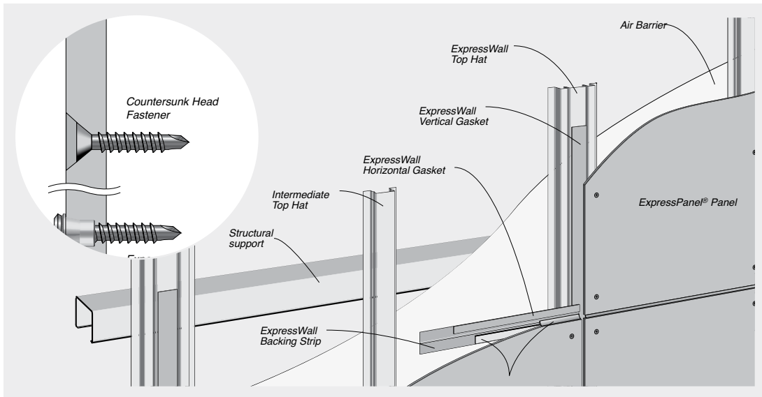
FIGURE 3.09 System Overview
